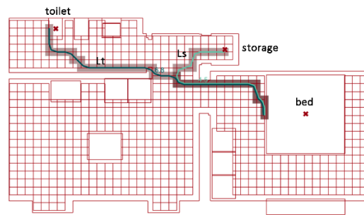
Figure 2 : An example of how the shortest paths between important points on a grid are calculated.
