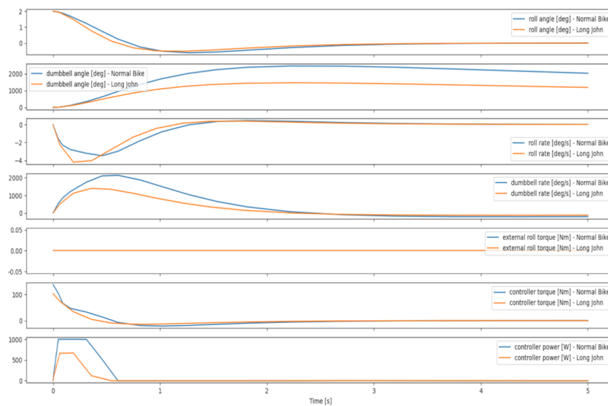
Figure 2: Roll stabilization results at zero speed from an initial roll angle of 2^\circ for a regular bicycle and a cargo bicycle.
