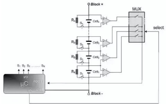
Fig. 9. Cell Balancing
