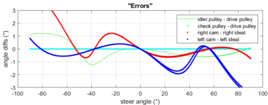
Figure 3. Steer angle errors.
