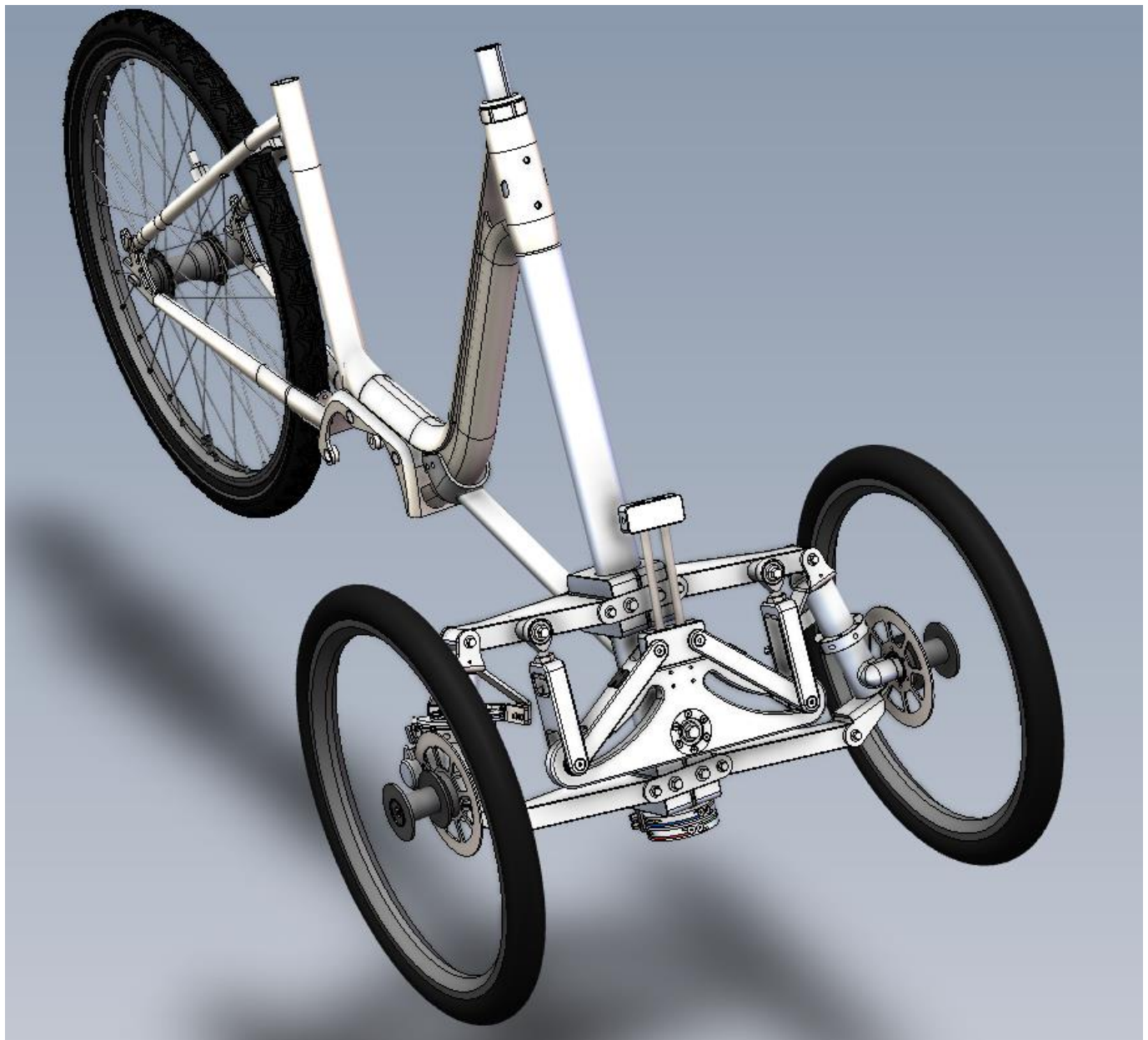
Figure 5. Final design solid model.
