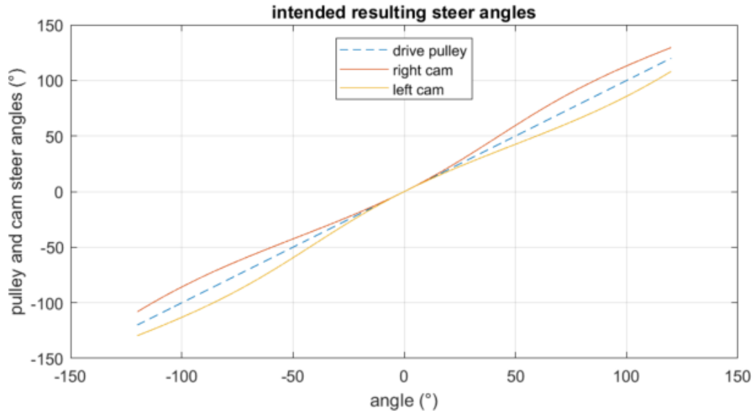
Figure 2. Resulting steer angles.
