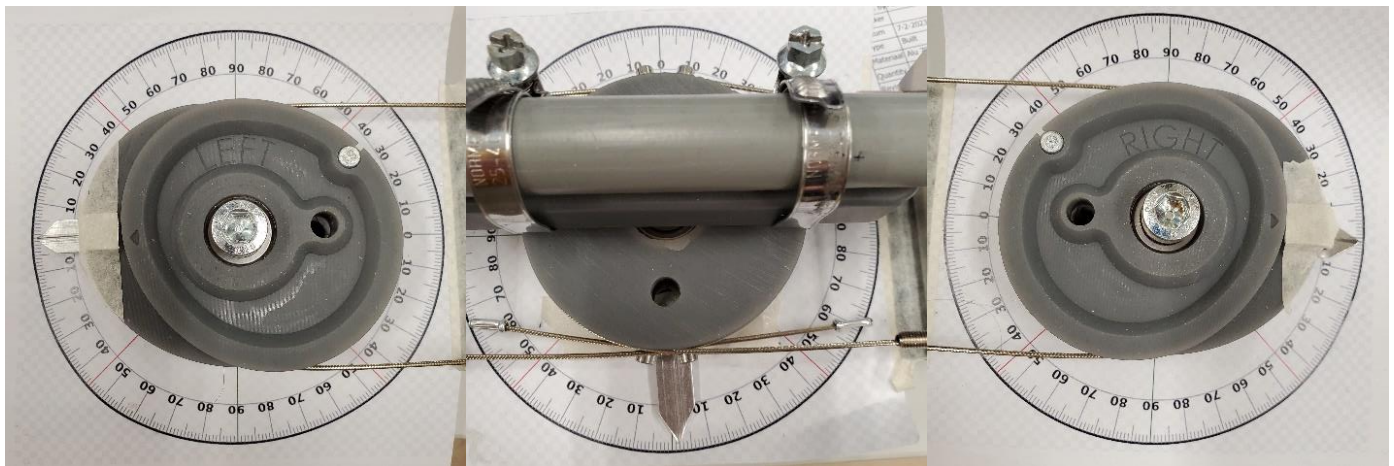
Figure 4. Images of the cable and cam steering system 3D-printed prototype.
