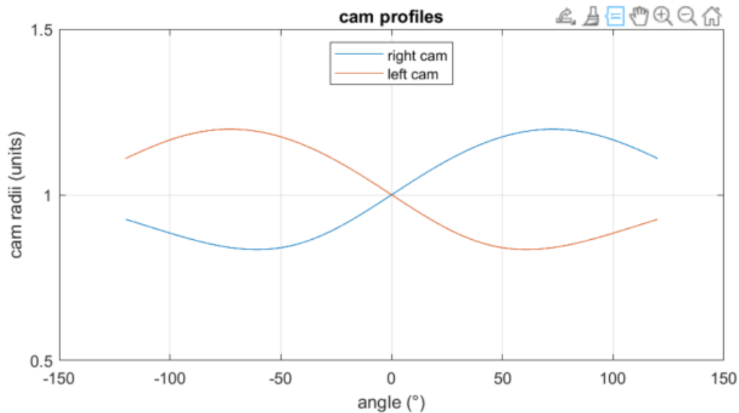
Figure 1. Steering cam profiles.
